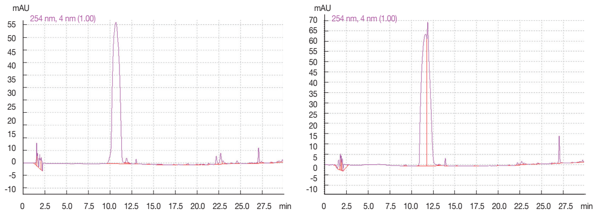
Supplementary Fig. S1. Chromatograms of brucine (a) and strychnine (b) at concentrations of 100.5 and 99.9 ppm, respectively.
