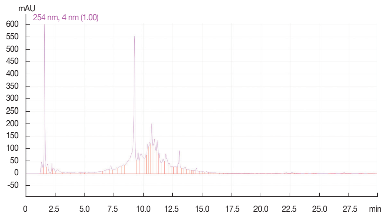
Supplementary Fig. S2. Chromatogram of Strychnos ligustrina extracts at 5,080 ppm concentration.
